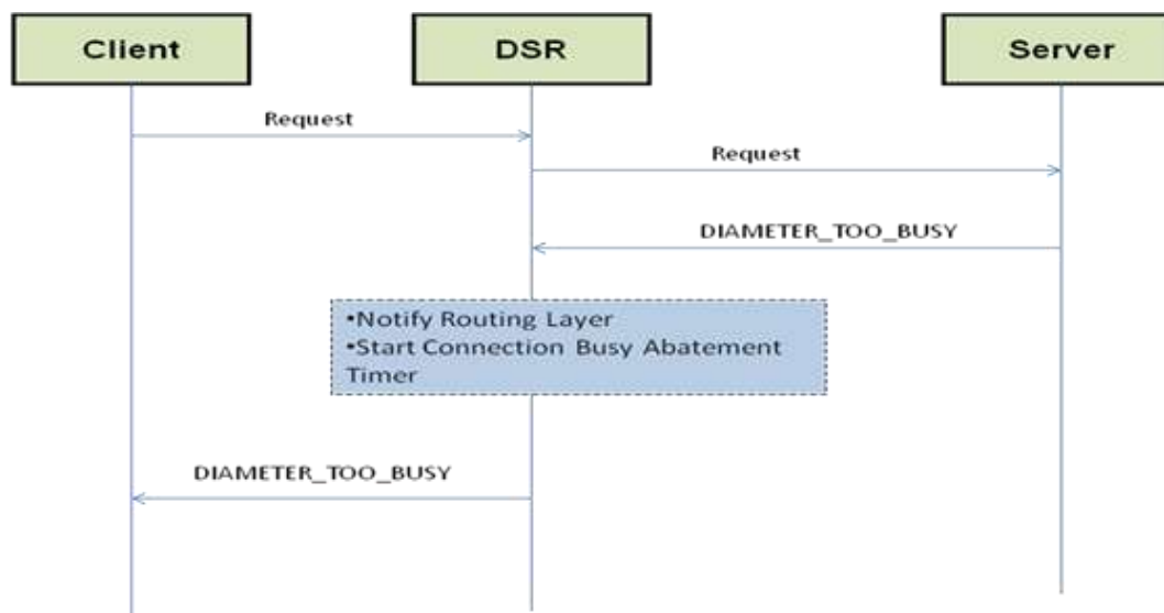
Figure 27 – Connection Busy
