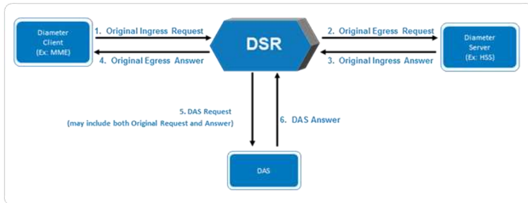
Figure 64 - Message Copy Overview
