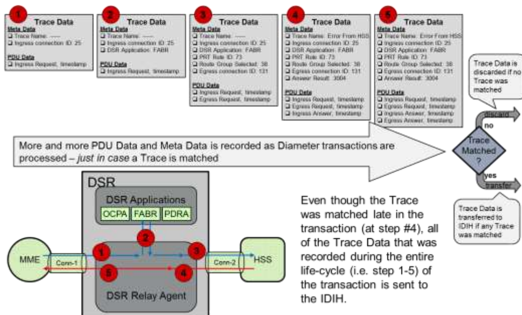
Figure 67 - IDIH Trace Data
