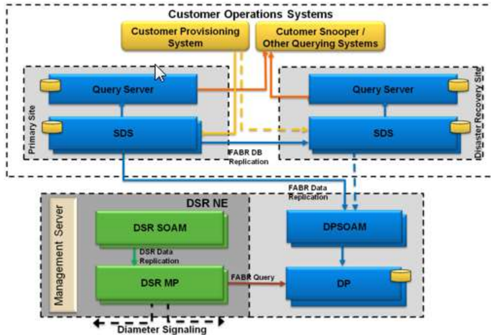
Figure 52 - Subscriber Data Server Architecture
