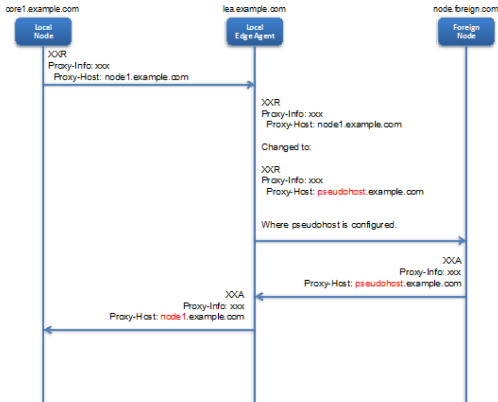
Figure 51 - Proxy-Host Topology Hiding Message Flow
