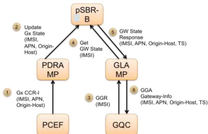
Figure 62 - IMSI Query with Single Matching Gx Session Use Case
