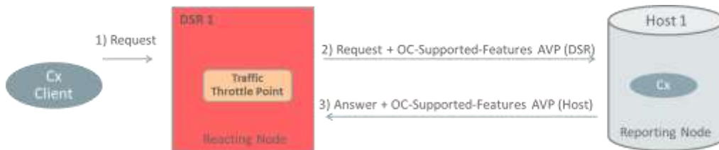
Figure 30 - DOIC Capabilities Announcement
