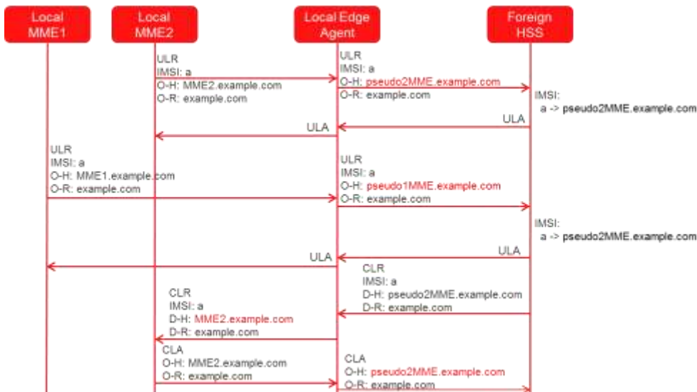
Figure 48 - MME/SGSN Topology Hiding
