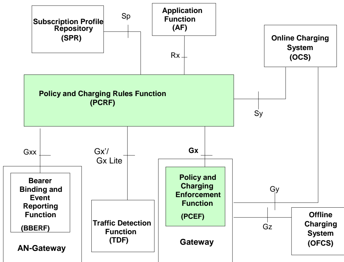
Figure 57 - Overall PCC logical architecture (non-roaming)
