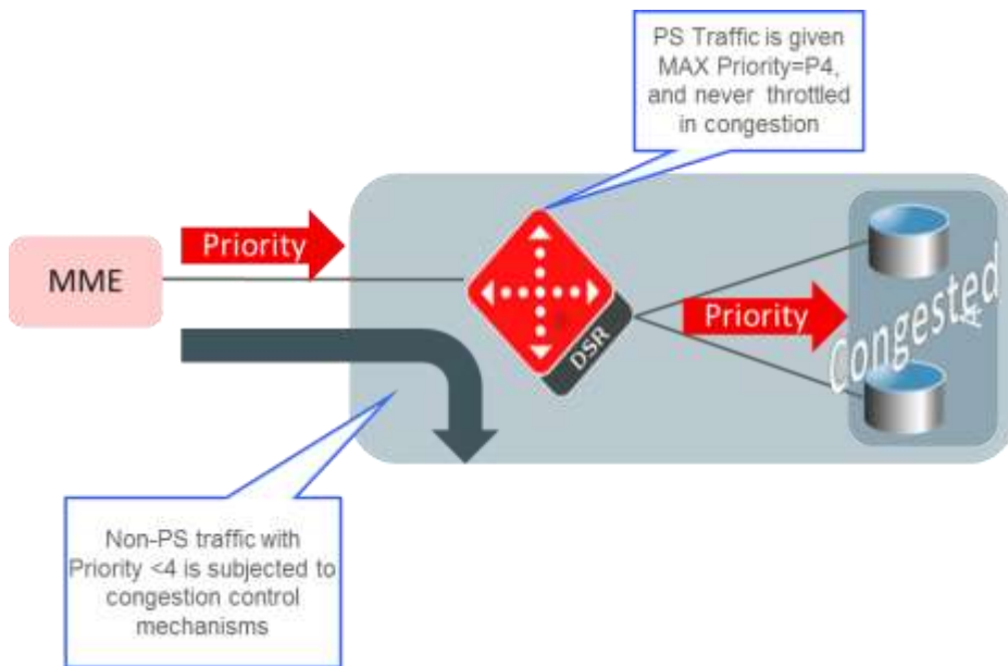
Figure 40 - NGN-PS Support
