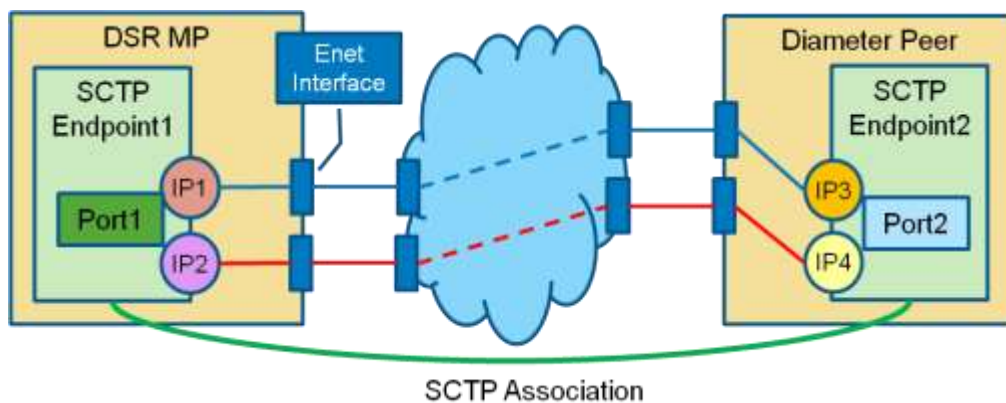
Figure 15 - SCTP Multi-Homing
