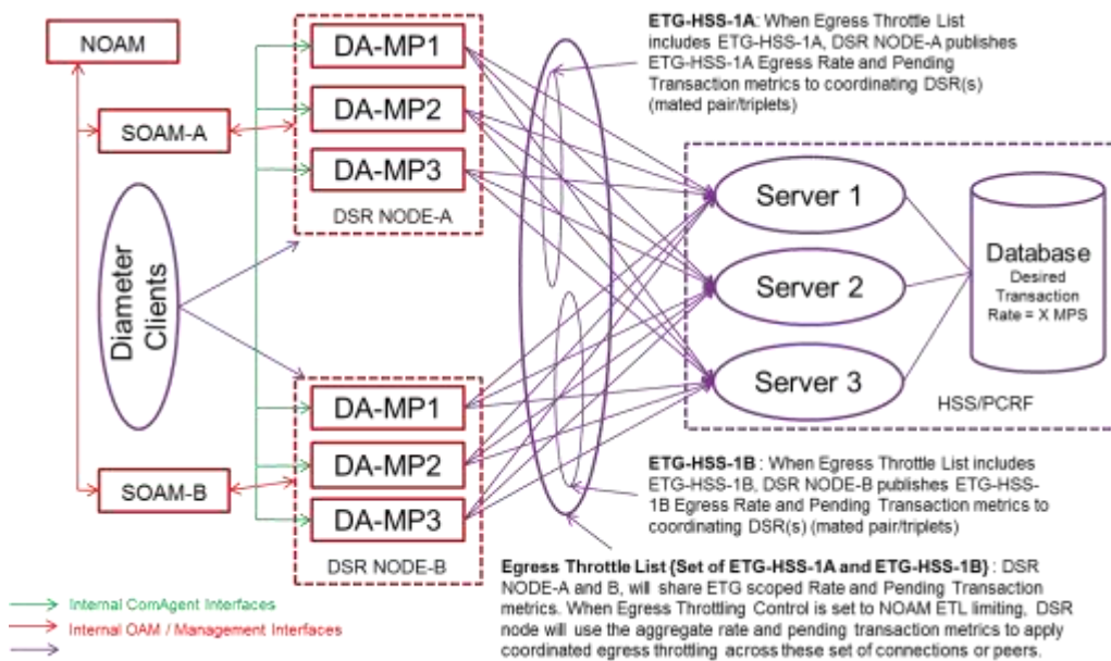
Figure 26 – 2 DSR Sites: Coordinated Egress Throttling Example
