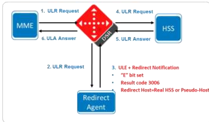
Figure 14 - Redirect Agent
