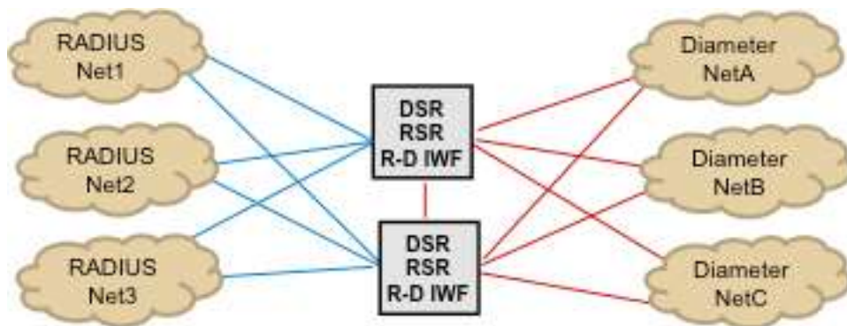
Figure 45 - RSR and R-D IWF Deployment
