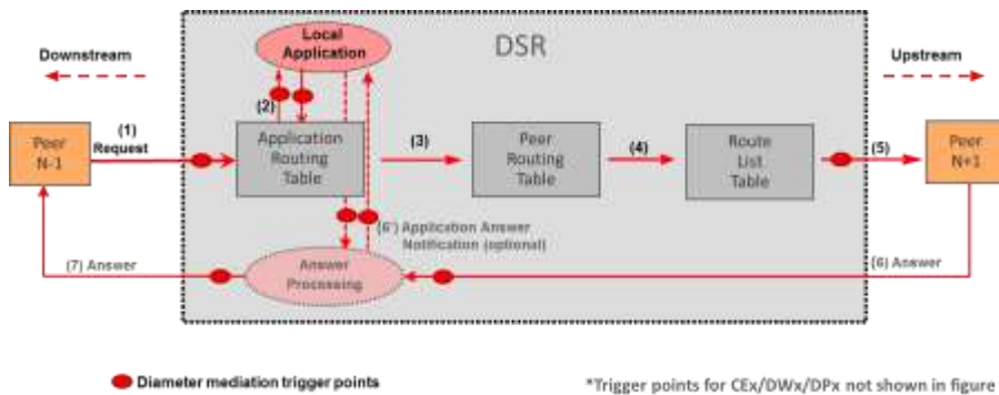
Figure 47 - Mediation Trigger Points
